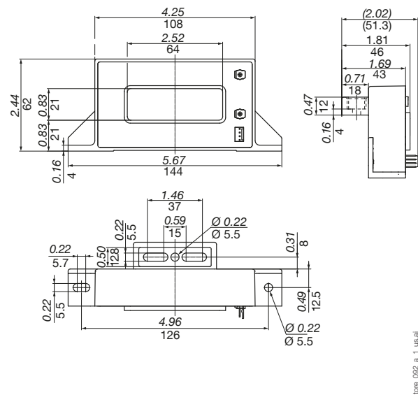
Solid-core sensors 850 ... 5000 A (frame size 2)
