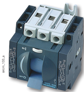
Toggle switch SIRCO M2 3x80A + 2 auxiliary contacts
